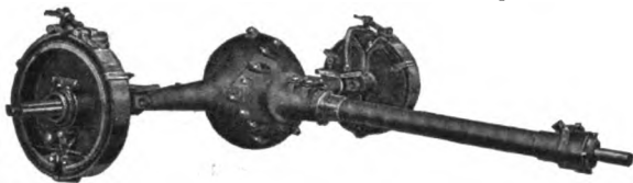
This is the Axle No. 525 Timken Rear
